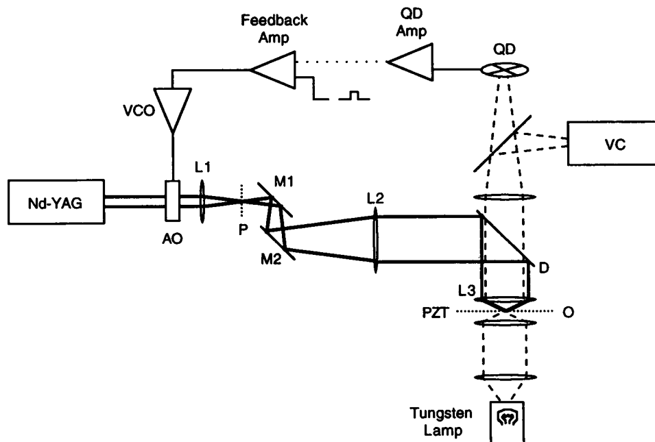
FIGURE 1 Schematic diagram of the optical trap and detection system. The solid lines represent the path of the Nd-YAG laser. The dashed lines represent the illuminating light from a tungsten lamp. Optics include lenses ( L_1 , L_2 ), mirrors ( M_1 , M_2 ), a dichroic filter ( D ), and a microscope objective ( L_3 ). The laser beam can be shifted in the plane of the specimen ( O ) by deflecting it with two orthogonally mounted acousto-optic modulators ( AO ) and by moving the mirrors M_1 , M_2 . The illuminating light is split between a video camera ( VC ) and a quadrant photodiode detector ( QD ), which indicates the position of a trapped bead. The feedback loops can be closed by feeding the output signals from the quadrant detector into the driver circuits for the voltage-controlled oscillators ( VCO ), which control the acousto-optic modulators.
