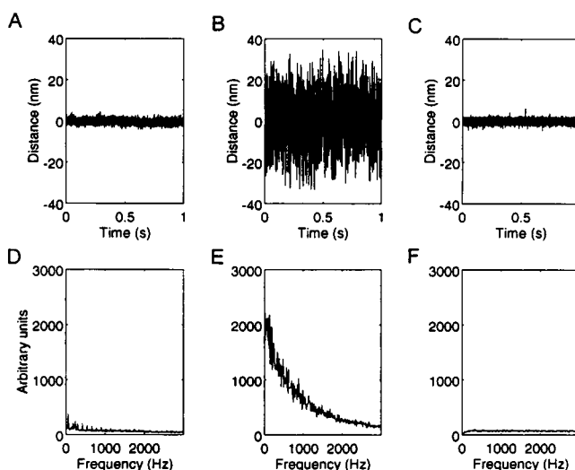
FIGURE 12 Positional noise on a 1-μm diameter bead (A) immobilized on a coverglass surface, (B) held without feedback in a laser trap with a stiffness of 0.04 \text{ pN} \cdot \text{nm}^{-1} , and (C) held in the same laser trap with feedback control. (D–F) Fourier transform spectra of the positional noise corresponding to A–C, respectively. Detector bandwidth was 5 kHz.
