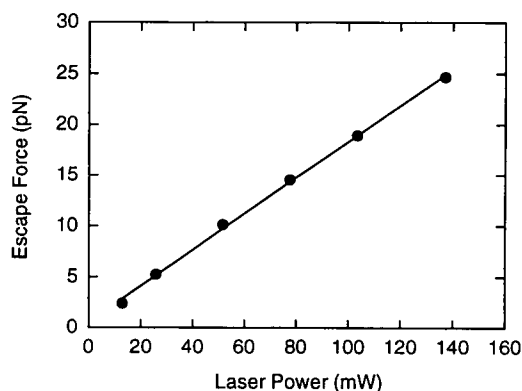
FIGURE 7 Escape force for a trapped bead (1- \mu m diameter) as a function of laser power. The escape force represents the maximum force an optical trap can exert to keep a bead trapped.
