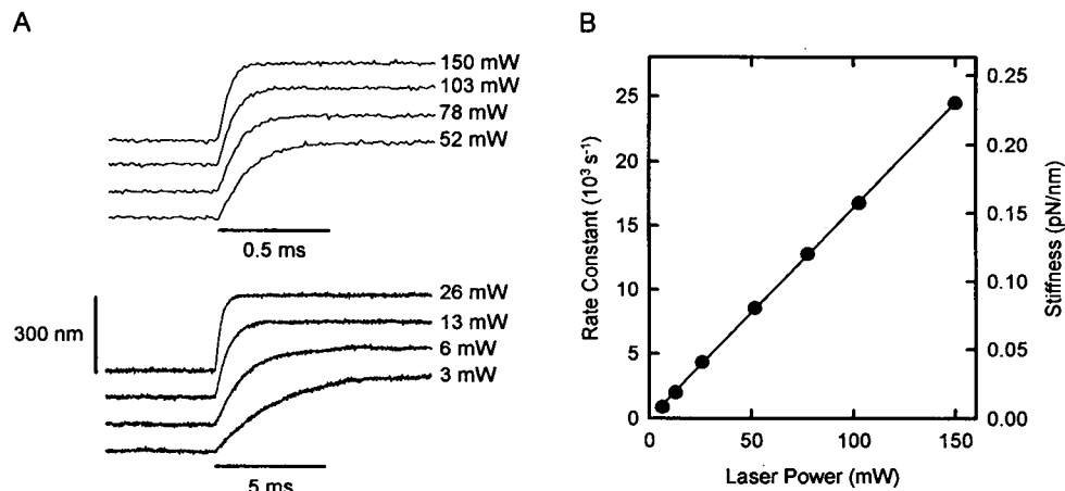
FIGURE 4 (A) Response of a trapped bead (1- \mu\text{m} diameter) to rapid trap displacements of 300 nm at laser powers ranging from 3 to 150 mW. For laser powers of 52 to 150 mW the response is shown on an expanded time scale. Detector bandwidth was 20 kHz (single-pole, low-pass filter). Each trace is an average of 100 data sweeps. (B) The rate constant of the bead response as a function of laser power.
