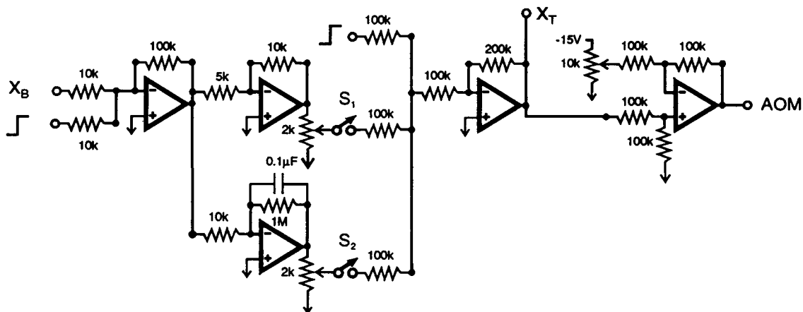
FIGURE 2 (A) Block diagram of one channel of electronic circuits showing feedback arrangements. The pulse inputs were used to open and close the feedback loop. (B) Quadrant detector circuit. The feedback resistors R had a switched range, 10 k \Omega to 200 M \Omega . Operational amplifiers: first stage, OPA121; second stage, OP270; final stage, AMP03. (C) Feedback amplifier circuit (one channel). Operational amplifiers: OP27. S_1 , S_2 ; analog switches used to open and close the feedback loop. Pulse inputs were used to deflect the laser beam.
