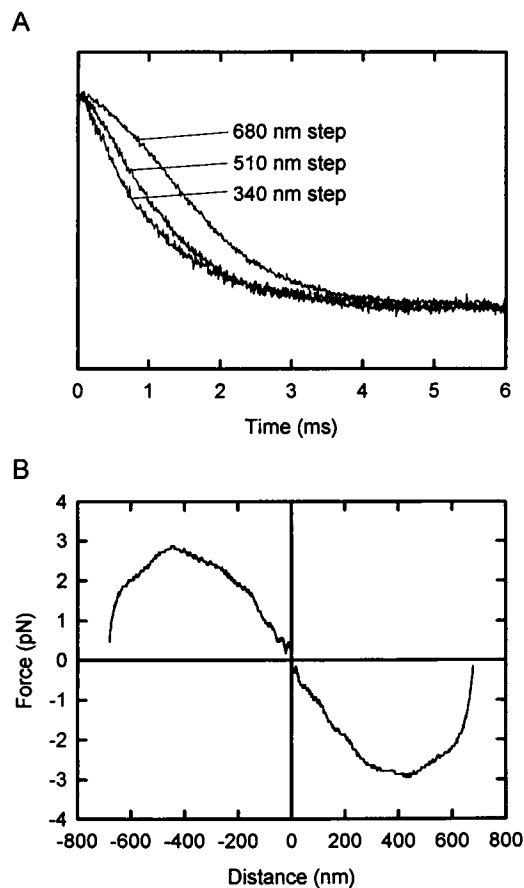
FIGURE 5 (A) Time course of the response of a trapped 1-μm-diameter bead for rapid trap displacements of 340, 510, and 680 nm. The responses are normalized to fit on the same scale to illustrate the lag in the response for large trap displacements. Detector bandwidth was 20 kHz (single-pole, low-pass filter). Each trace is an average of 100 data sweeps. (B) Force profile of an optical trap as a function of displacement of a bead from the center of the trap. The force was calculated by differentiating the bead response to a large trap displacement and calculating the viscous (Stokes') force.
