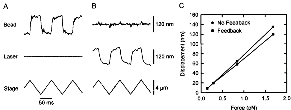
FIGURE 11 Optical trap stiffness calibration with and without feedback control. (A) Without feedback: the response of a trapped bead to a triangular wave input to the microscope stage position (see Fig. 6). (B) With feedback: the laser trap position now shows the response. (C) Displacement measured from bead position trace (without feedback) and from trap position trace (with feedback), as a function of applied force. Detector bandwidth was 100 Hz (single-pole, low-pass filter). Each trace is an average of 100 data sweeps.
